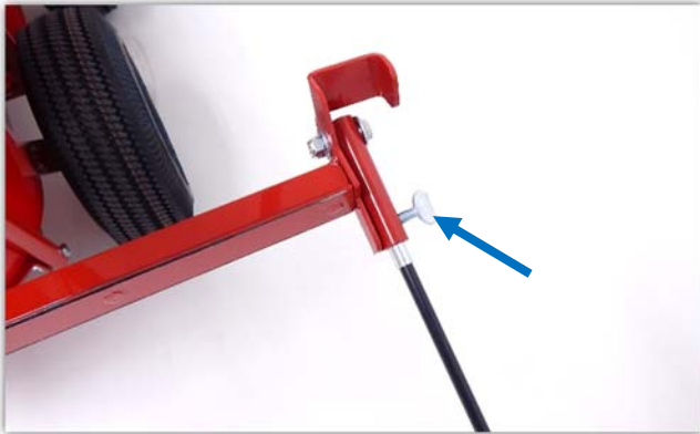
Step 2: Insert the line guide into the barrel and secure with the provided thumb screw.
