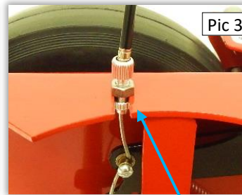
Cable Adjuster Correct Position
